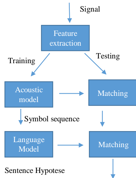
Figure 3 Speech recognition process
